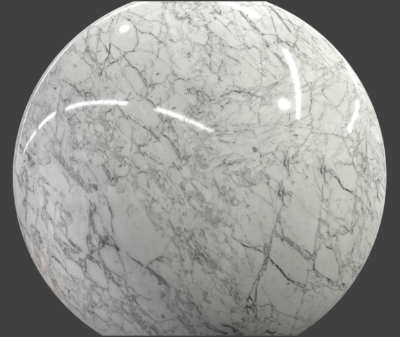
Marble Stone
