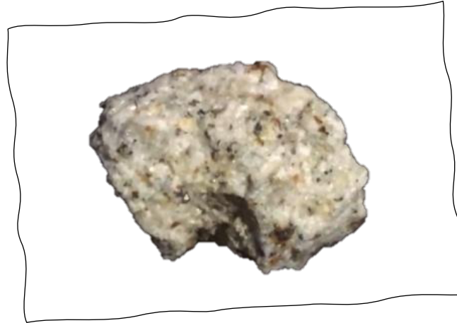
Sandstone
