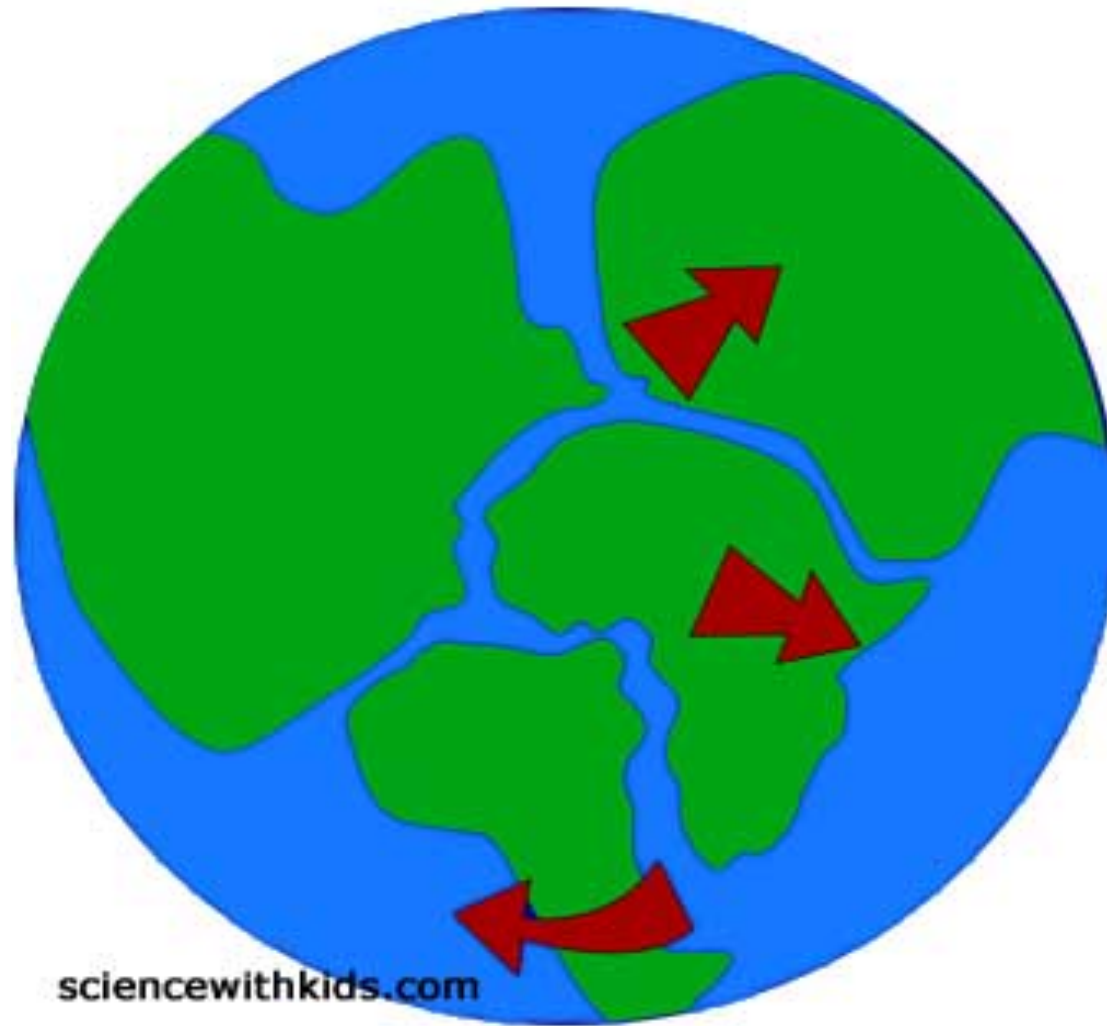
Plate tectonics
