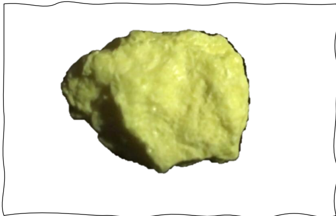
Sulphur mineral
