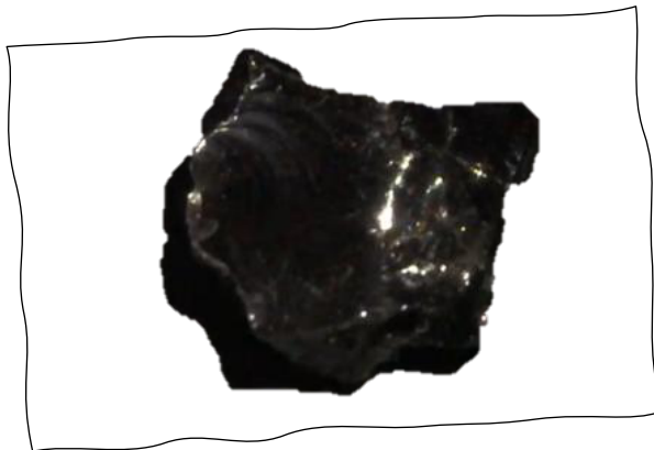
Obsidian
